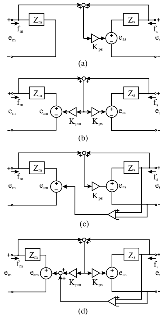
Fig. 2. Telemanipulation Controller Architectures (Two-Port Representations): (a) position forward (PF), (b) position exchange (PE), (c) position forward/force feedback (PFFF), and (d) position exchange/force feedback (PEFF).
