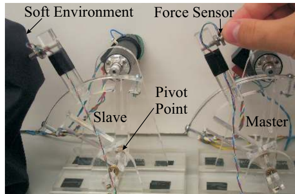
Fig. 1. Experimental system.
