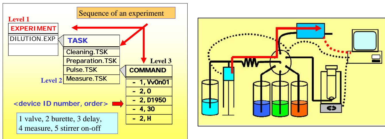
Figure 4. Illustration of the three software levels of instructions during a sequence of an experiment.
