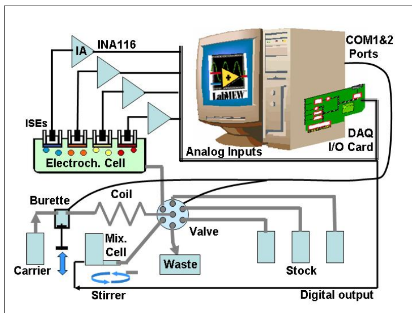
Figure 2. Manifold and hardware used for the developed automated e-tongue.
