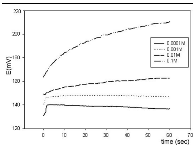
Figure 7. Transient recording of the response of one of the sensors after step changes to different automatically prepared solutions with different calcium concentration levels.
