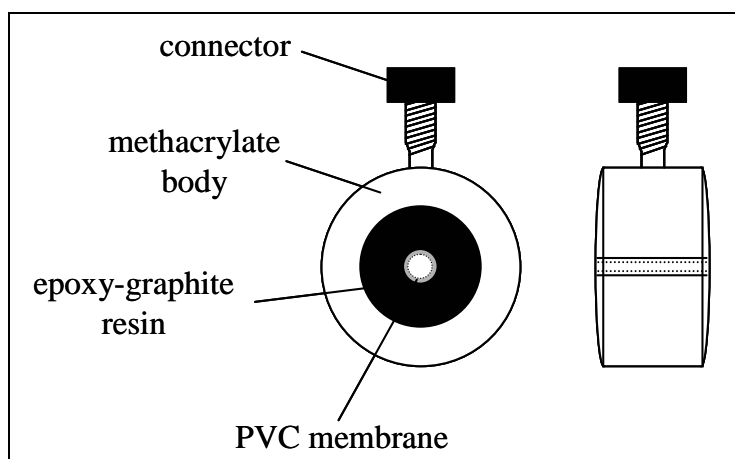
Figure 3. Design of the flow-through tubular electrode used in the SIA system.
