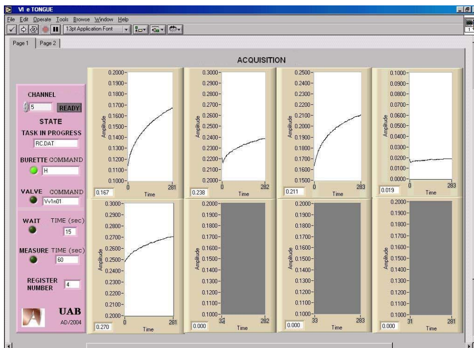
Figure 5. Front panel VI. Acquisition of 5 potentials during sensor transient response.
