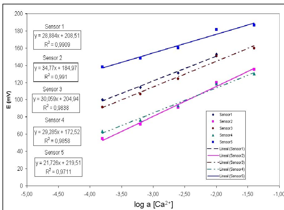
Figure 6. Example of an automated calibration run versus a single ion.
