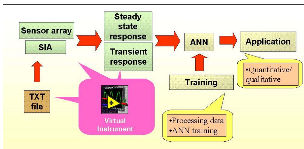
Figure 1. Design strategy for the automated SIA e-tongue.
