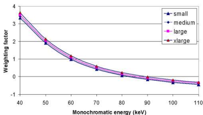
FIG. 7. Weighting factor for 80 kV image as a function of monochromatic energy for the four phantom sizes, where the effective energies of the low and high kV were different.
