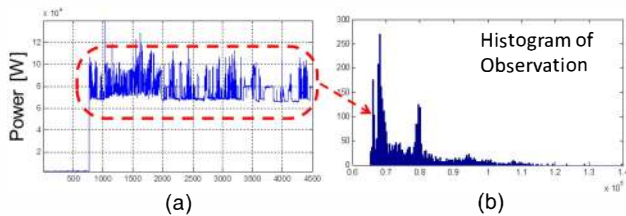
Fig. 3. Impulse Noise in Measured Power Data
