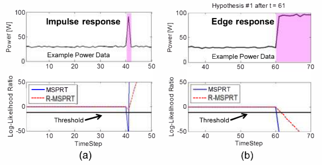
Fig. 7. Demonstration of RMSPT: (a) Impulse noise response and (b) True edge response
