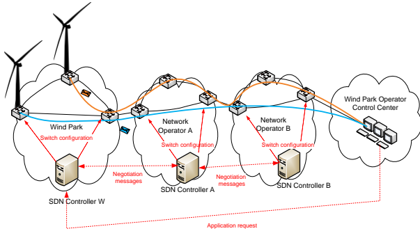
Figure 3: Inter-domain QoS negotiation
