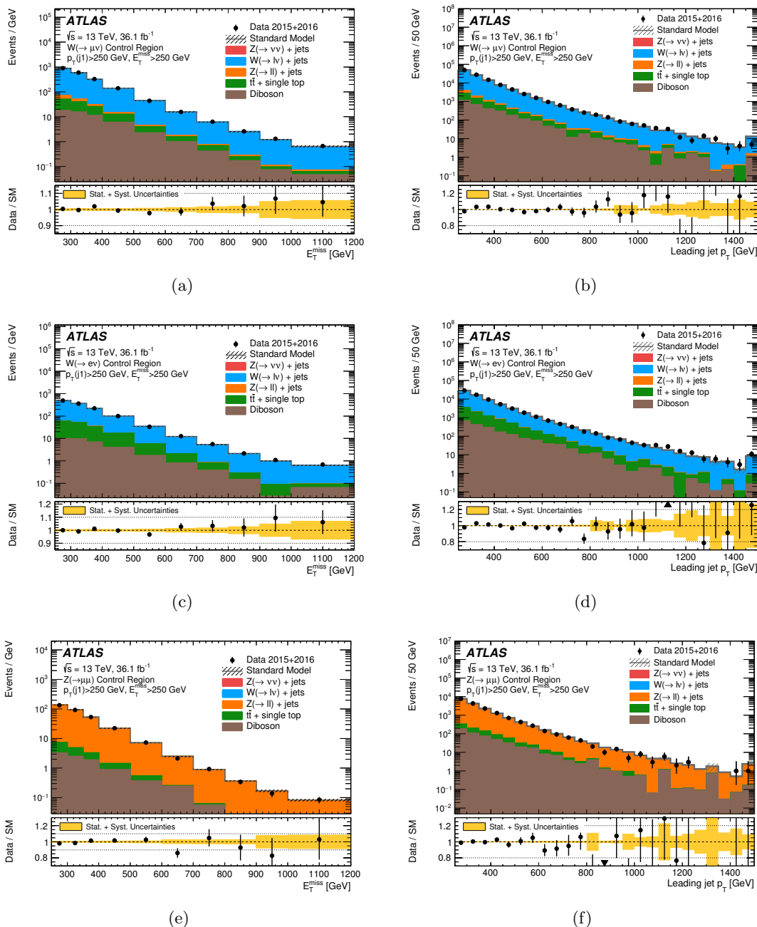
Figure 2. The measured (a),(c),(e) E_T^{\text{miss}} and (b),(d),(f) leading-jet p_T distributions in the W(\rightarrow \mu\nu) + \text{jets} , W(\rightarrow e\nu) + \text{jets} , and Z/\gamma^*(\rightarrow \mu^+\mu^-) + \text{jets} control regions, for the E_T^{\text{miss}} > 250 GeV inclusive selection, compared to the background predictions. The latter include the global normalization factors extracted from the fit. The error bands in the ratios include the statistical and systematic uncertainties in the background predictions as determined by the binned-likelihood fit to the data in the control regions. The last bin of the E_T^{\text{miss}} and leading-jet p_T distributions contains overflows. The contributions from multijet and non-collision backgrounds are negligible and are not shown in the figures.
