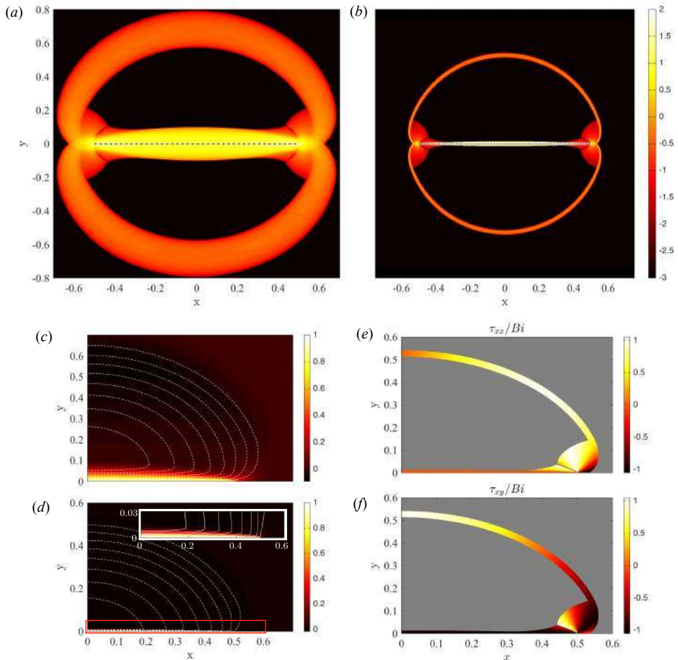
FIGURE 10. Flow around a plate of unit length for (a) Bi = 32 and (b) Bi = 2048 , showing density maps of \log_{10}(\dot{\gamma}) . The dashed line locates the plate, which is moving from left to right with unit speed. (c,d) Density maps of the corresponding horizontal velocity component (displaying one quarter of the plane due to symmetry) for (c) Bi = 32 and (d) Bi = 2048 . Dashed white lines show a selection of streamlines. The inset in (d) shows a magnification of the boundary layer flow against the plate, as indicated by the box of the main panel. (e,f) The normal and shear stress components, respectively, scaled by Bi , for Bi = 2048 . (g) Plug regions (shaded grey) for (left to right) Bi = 8 , Bi = 32 , Bi = 128 , Bi = 512 , and Bi = 2048 .
