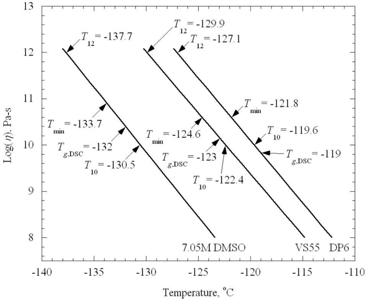
Figure 6. Best-fit results for viscosity as a function of temperature, where T_{12} denotes the temperature at which the viscosity extrapolates to a value of 10^{12} Pa-s, T_{\min} denotes the lowest temperature at which experimental data were obtained for that CPA, T_{g,DSC} denotes the glass transition temperature measured by differential scanning calorimetry (corresponding to the peak overshoot during rewarming), and T_{10} denotes the temperature at which the viscosity reaches a value of 10^{10} Pa-s.
