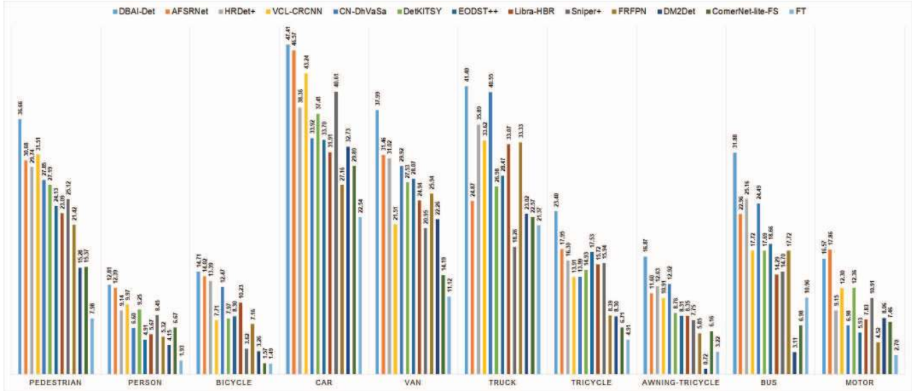
Figure 2. The average precision scores of the submitted detectors in each object category.
