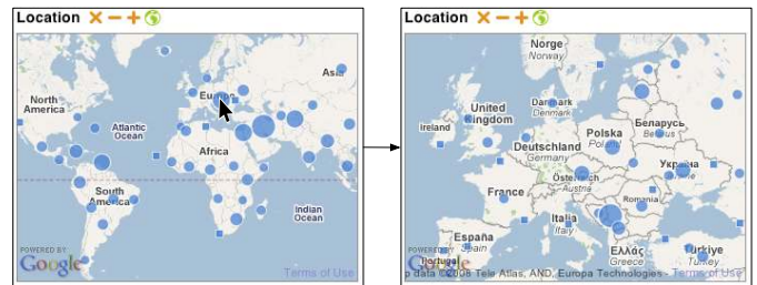
Fig. 2. Location VisGet: the size of a circle represents how many items refer to a region. Interacting with the map and the circles changes the spatial query parameter which is defined by the map's bounds.
