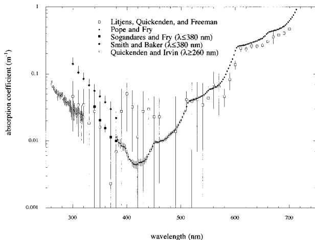
Fig. 1. Measurements of the absorption coefficient of pure water as a function of wavelength. In each case, error bars are those quoted by the respective authors.
