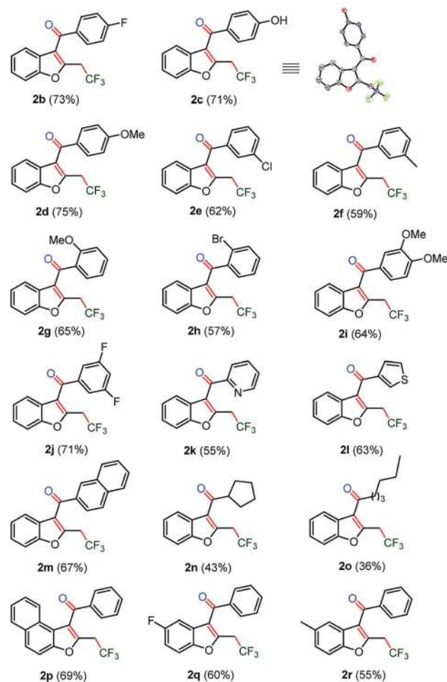
Scheme 2 \text{CF}_3 -Benzofurans: the scope with regards to the ethynyl and vinyloxy rings; the reactions were carried out at 0.1 mmol of 1a using 0.3 mmol of \text{CF}_3\text{SO}_2\text{Na} and 0.01 mmol of photocatalyst PQ in \text{CH}_3\text{CN} + \text{H}_2\text{O} (0.9 + 0.1 mL) under Ar, and the progress of the reaction was monitored by TLC for 4–8 h.
