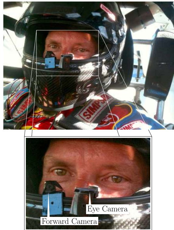
Figure 1. Early prototype for initial data collection in a NASCAR race circuit. This prototype consists of a forward facing camera to observe the environment from the driver’s point of view and an eye facing camera for estimation of the gaze direction. Both cameras are connected to a laptop computer for data recording.
