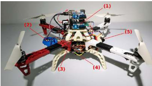
Fig. 8: The quadrotor used in our experiments. (1) The onboard computer running our algorithms. (2) The downward-looking camera used to detect the platform. (3) The PX4 autopilot. (4) The TeraRanger distance sensor. (5) The 45° angled-down camera used for visual odometry.
