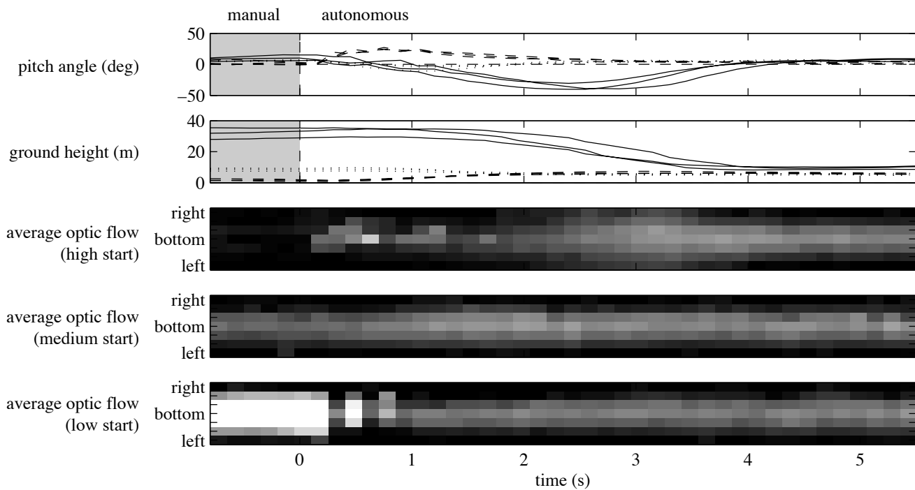
Fig. 21 Data recorded from the on-board sensors during the altitude regulation experiments with the real platform. Nine flights are shown, during which the aircraft was manually controlled (grey background) at an altitude of either about 2 m (dashed lines), 10 m (dotted lines) and 30 m (solid lines), before activating optiPilot at t = 0 . The pitch angle and altitude of each flight is plotted, as well as the average translation-induced optic flow perceived in each viewing direction when started from each of the three altitudes.
