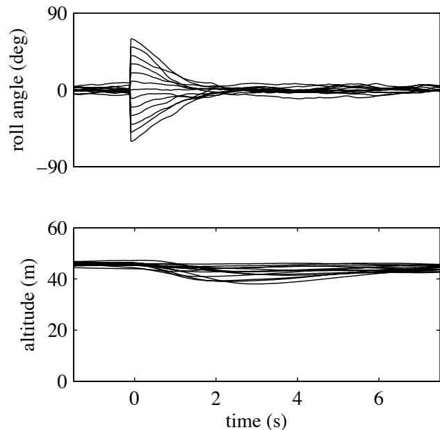
Fig. 16 Roll angle (top) and altitude (bottom) profiles of the simulated platform during roll angle perturbation experiments. The aircraft was initially in stable and level flight. At t = 0 , the aircraft was rotated by an angle ranging from -60^\circ to 60^\circ (with 10^\circ intervals) around its roll axis (the 13 profiles are represented). In all cases, the roll angle is regulated back to a level attitude in less than 1 s, with variations of altitude of approximately 8 m in the worst cases.
