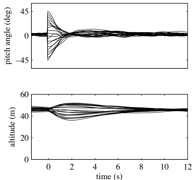
Fig. 15 Pitch angle (top) and altitude (bottom) profiles of the simulated platform during pitch angle perturbation experiments. The aircraft was initially in stable and level flight. At t = 0 , the aircraft was rotated by an angle ranging from -45^\circ to 45^\circ (with 5^\circ intervals) around its pitch axis (the 19 profiles are represented). The pitch angle was regulated within about 3.5 s back to the small positive value required to generate lift for level flight, with variations of altitude of approximately 10 m in the worst cases.
