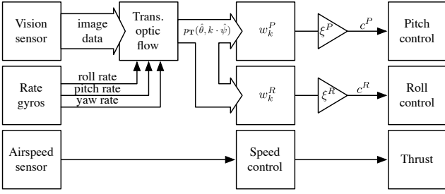
Fig. 6 The complete optiPilot control architecture. Data from the vision system and rate gyroscopes is used to extract translational optic flow (section 3.1). Optic flow measurements p_{\mathbf{T}} are then linearly combined using two sets of weights w_k^P and w_k^R , corresponding to pitch and roll control (section 3.3). In parallel, the thrust is controlled by a simple regulator to maintain cruise speed, based on measurements from an airspeed sensor.
