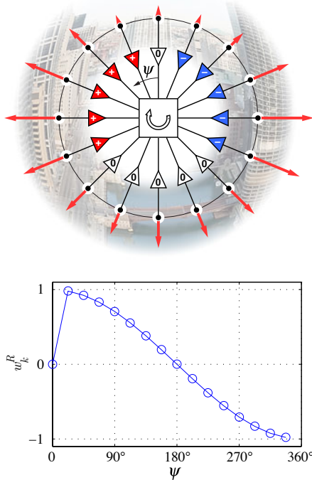
Fig. 8 ( top ) Possible distribution of w_k^R for the generation of the roll control signal. The arrow in the centre indicates roll direction for a positive roll signal. ( bottom ) Example weight distribution according to (5).
