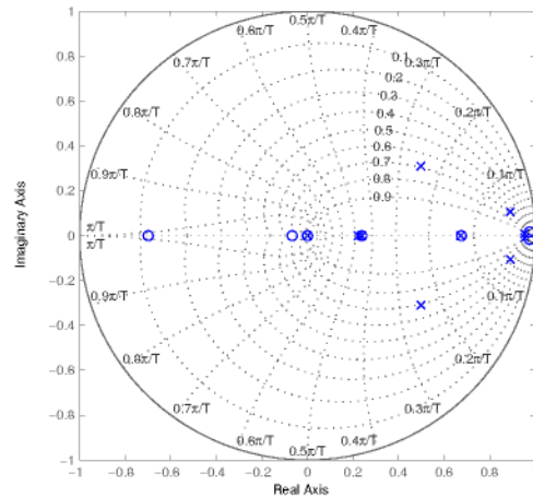
Fig. 7. Pole-zero map of the closed-loop system for x or y. Except for the four poles induced by the time delay all poles lie within 1-30 rad/s. No pole has a damping lower than 0.5. A zero situated at -7.2 is not displayed on the plot.
