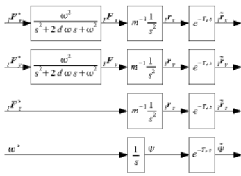
Fig. 5. The four decoupled linear systems. They were obtained by transforming the system inputs of Fig. 4 and exchanging the order of the nonlinear input transformation and the second order system blocks. This can be justified by the smoothness of the nonlinear transformation and the high speed of the second order system.
