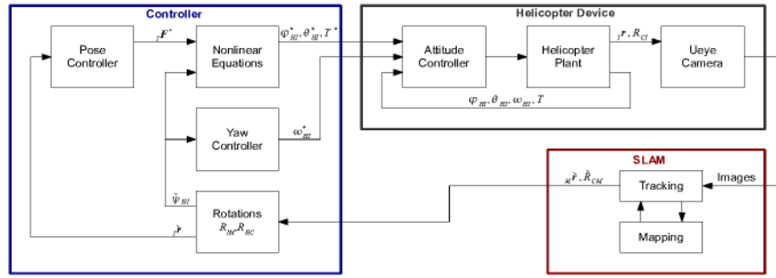
Fig. 10. Closed-loop controller structure. The entire data flow is represented. Receiving the images from the mounted camera the SLAM algorithm computes the estimate of the pose of the camera. This is transformed into the position and yaw angle of the helicopter in the inertial frame and fed to the controller. After the nonlinear control input transformations (Eq. (4),(5),( 6)) the reference values are sent back to the attitude controller on the quadrotor.
