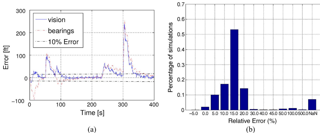
Fig. 6. Open-loop comparison of the Aidal and Hammel EKF to the proposed EKF with pointwise maneuvers of the lead aircraft. (a) Depicts a sample plot of the estimation error versus time and (b) shows the relative L_2 -norm error difference between the original and modified EKF algorithms as a percentage of 1000 simulations as a probability density. The NaN entry means that the Aidal and Hammel EKF failed to estimate; this happened for approximately 6% of the runs. The median performance difference for bearings-only EKF is 30% worse (assuming convergence occurs).
