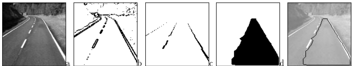
Figure 11: Lane detection on a straight road: (a) input image; (b) image obtained by thresholding the gradient image; (c) image obtained by the perspective-based filter; (d) stretched template; (e) superimposition of the edges of the stretched template onto the original image. In this case both the thresholded gradient (b) and the perspective-based filtered (c) images can be used as input to the DT.
