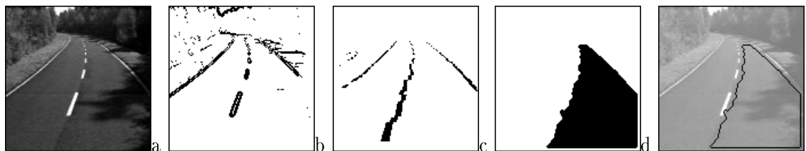
Figure 12: Lane detection on a curved road: also in this case both the thresholded gradient (b) and the perspective-based filtered (c) images can be used as input to the DT.
