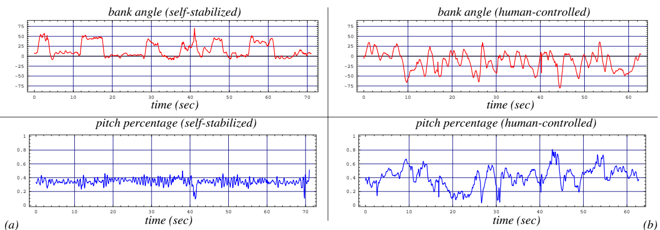
Fig. 5: (a) Bank angle and pitch percentage for a self-stabilized flight (sequence of level-flight and left-turn segments), and (b) bank angle and pitch percentage for typical human-controlled flight.
