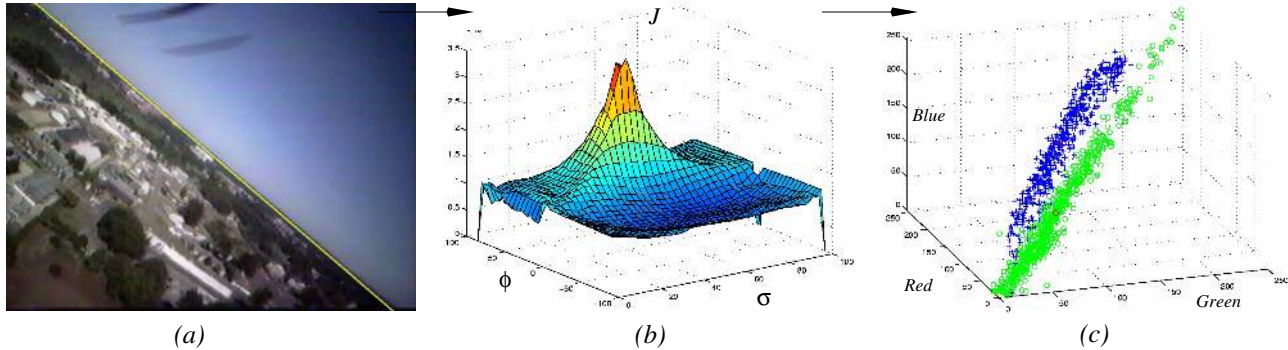
Fig. 3: (a) original image, (b) optimization criterion as a function of bank angle and pitch percentage and (c) resulting classification of sky and ground pixels in RGB space.
