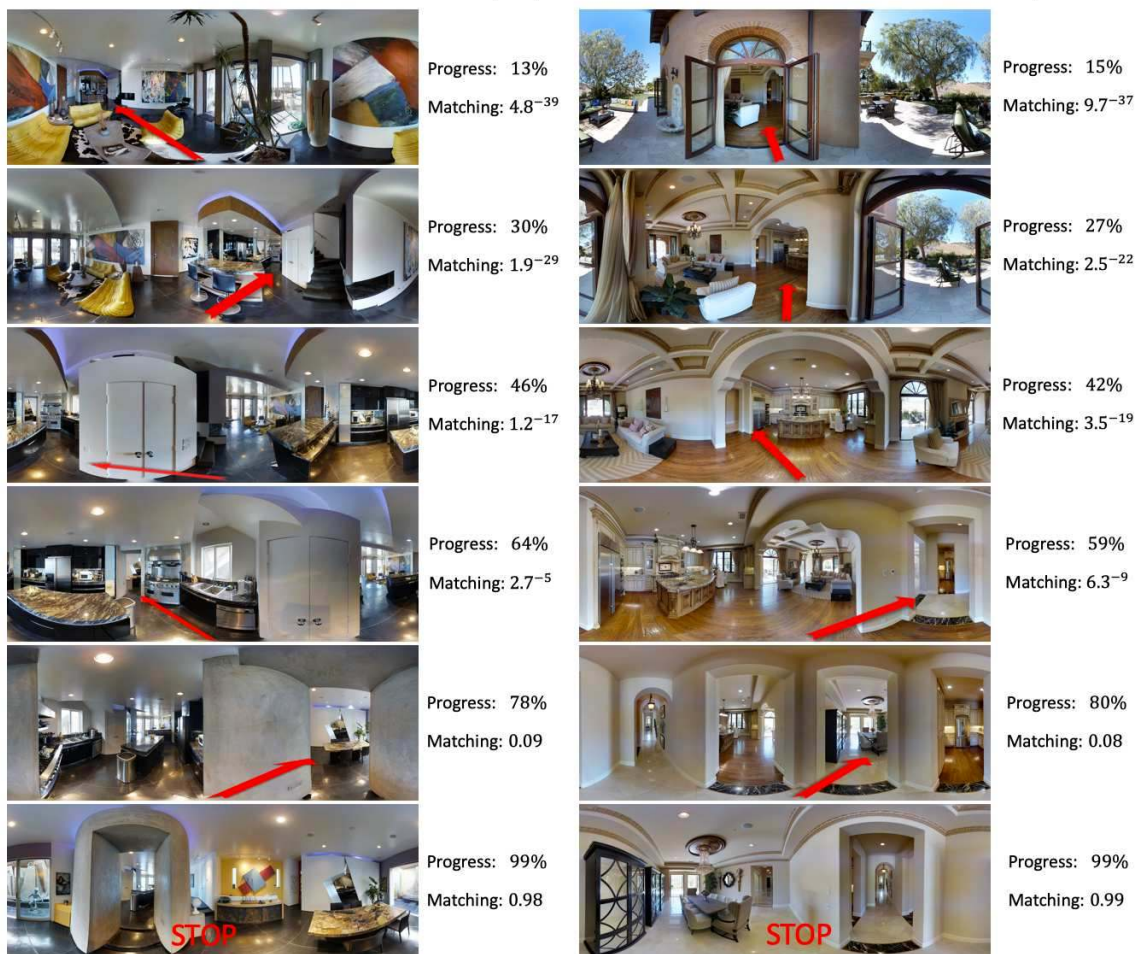
Figure 4. Visualization process of two trajectories in testing. Two complex language instructions are shown in top boxes. Each image is a panoramic view, which is the vision input for AuxRN. Each red arrow represents the direction to the next step. For each step, the results progress estimator and the matching function are shown as left.
