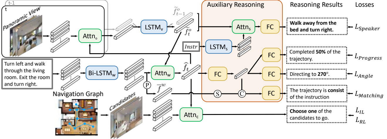
Figure 2. An overview of AuxRN. The agent embeds vision and language features respectively and performs co-attention between them. The embedded features are given to reasoning modules and supervised by auxiliary losses. The feature produced by vision-language attention is fused with the candidate features to predict an action. The “P”, “S”, and “C” in the white circles stand for the mean pooling, random shuffle and concatenate operations respectively.
