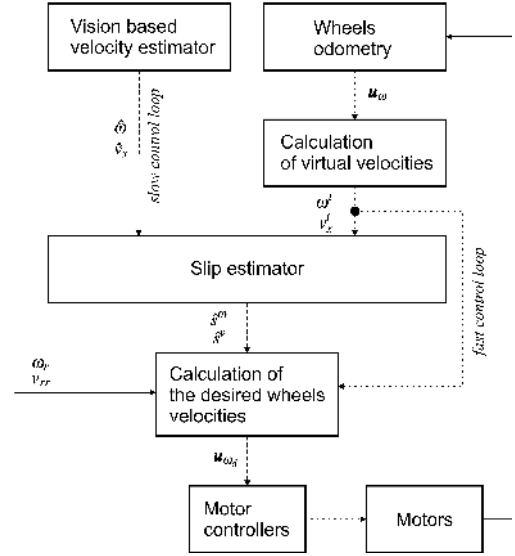
Fig. 11. Structure of the control system for SSMR with velocity and slip estimators
