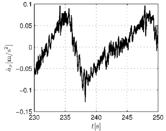
Fig. 10. Estimated accelerations
