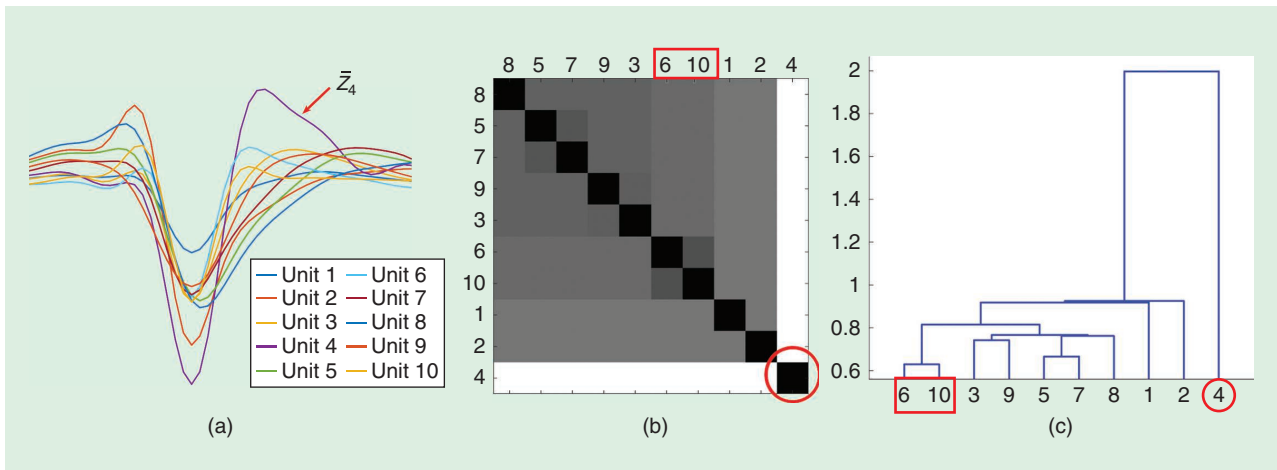
Figure 6. The iVAT as a visualization of SL clusters and dendrogram: (a) X_{10} \sim 10 waveforms, (b) the iVAT image of D_\varepsilon(X_{10}) , and (c) the SL dendrogram of X_{10} . (Source: Mahallati et al. [35].)
