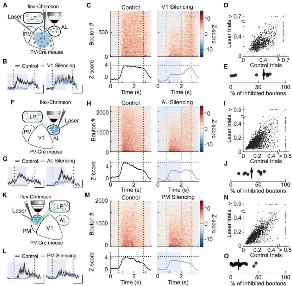
Figure 3. Functional influence of cortical inputs on LP pathways
