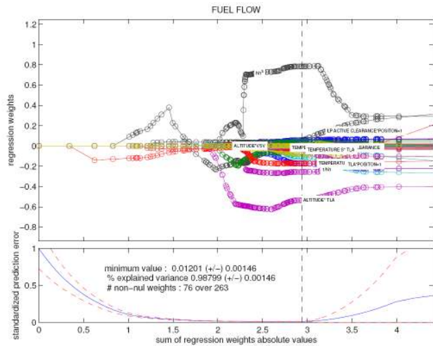
Figure 2: Selection of input combinations X of context measurements that impacts the evolution of fuel flow. The abscisse is the value of the constraint C . The top graph gives the coefficients \lambda . The bottom graph shows the evolution of the MSE. The vertical dashed line points the energie that was selected.
