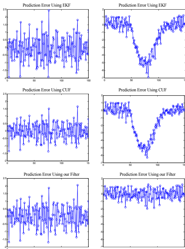
Figure 5. Prediction errors (between prediction and ground truth) of an EKF predictor,
