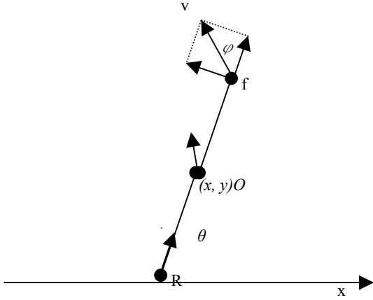
Figure 2. The bicycle model of car motion
