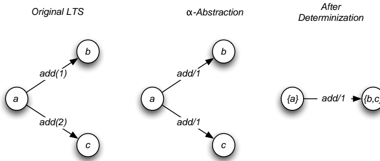
Fig. 2. Illustrating the DFA-Abstraction Algorithm.
