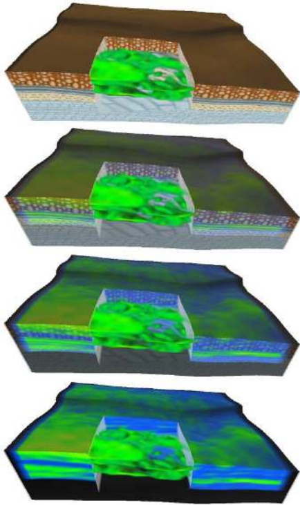
Figure 8: Blending from illustrative rendering to uninterpreted data rendering for seismic volumetric reflection data. [PGTG07].
