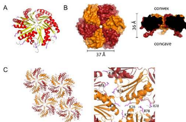
Figure 1. Crystal structure of the HO BMC-H. (A) HO BMC-H adopts the characteristic \alpha/\beta BMC-H fold (strands in yellow, helices in red). Edge residues K28 and R78 are shown as sticks. (B) Surface top and center sliced view with edge and thickness dimensions. The hexamer has a pronounced sidedness with distinct convex (top) and concave (bottom) surface. Protomer chains are alternately colored dark red and orange. (C) The hexamers pack into uniformly oriented layers in the crystal. Close-up view on the right shows residues K28 and R78 interacting at the interfaces (shown as magenta sticks).
