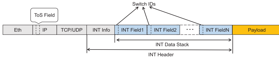
FIGURE 2. Packet format for realizing flexible ML-INT.
