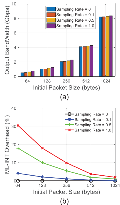
FIGURE 7. Measurements at the output of Switch 2 regarding (a) bandwidth, and (b) ML-INT overhead, when different initial packet sizes and sampling rates are considered.
