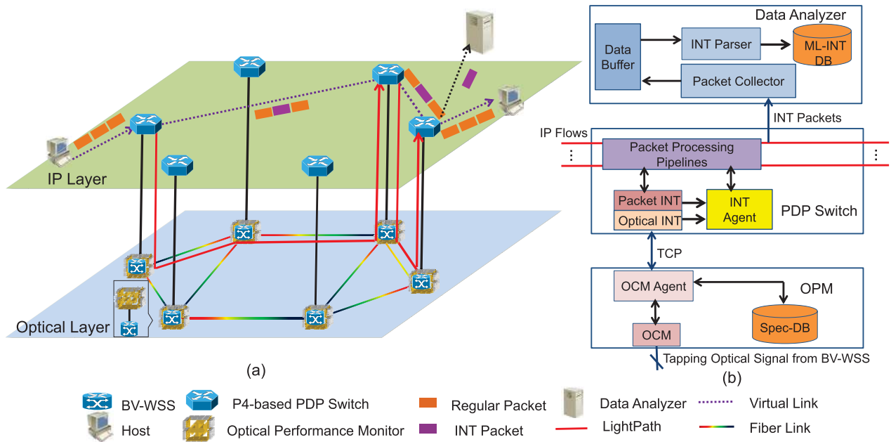
FIGURE 1. System architecture of flexible ML-INT system, BV-WSS: Bandwidth-variable wavelength selective switch, OPM: Optical performance monitor, OCM: Flex-grid high resolution optical channel monitor, ML-INT DB: Multilayer INT database, Spec-DB: Optical spectrum database.
