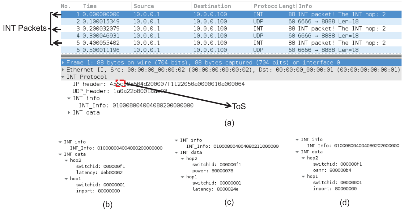
FIGURE 6. Wireshark captures to verify functionalities of our flexible ML-INT system, (a) packets captured at the Switch 2, (b) INT header of the first INT packet, (c) INT header of the second INT packet, and (d) INT header of the third INT packet.
