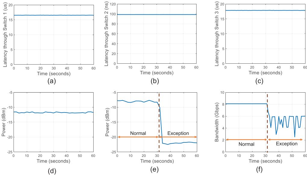
FIGURE 10. Results for the second use-case, (a) packet queuing latency at Switch 1 , (b) packet queuing latency at Switch 2 , (c) packet queuing latency at Switch 3 , (d) power of lightpath terminated at Switch 2 , (e) power of lightpath terminated at Switch 3 , and (f) end-to-end bandwidth measured by commercial traffic analyzer.
