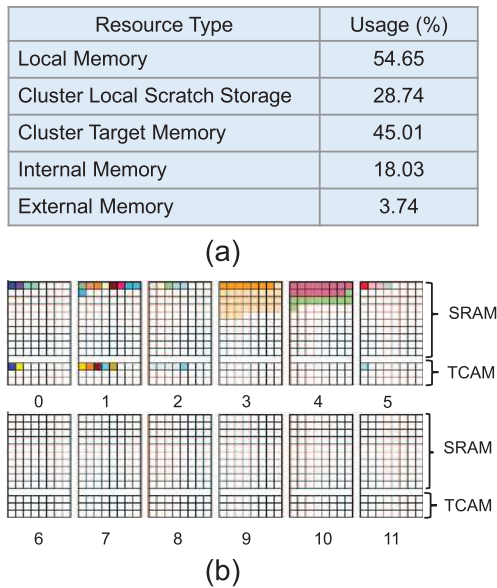
FIGURE 4. Memory resource utilizations of our ML-INT implementation on (a) SmartNIC, and (b) programmable ASIC switch.
