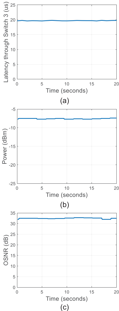
FIGURE 8. Realtime statistics provided by the data analyzer regarding (a) packet queuing latency through Switch 3 , and (b) power and (c) OSNR of Lightpath B-C , when the arrival rate of INT packets is 2 Mpps.
