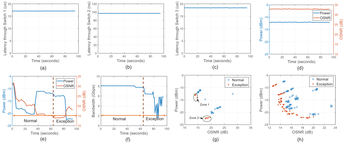
FIGURE 11. Results for the third use-case, (a) packet queuing latency at Switch 1, (b) packet queuing latency at Switch 2, (c) packet queuing latency at Switch 3, (d) power and OSNR of lightpath terminated at Switch 2, (e) power and OSNR of lightpath terminated at Switch 3, (f) end-to-end bandwidth measured by commercial traffic analyzer, (g) INT data regarding the correlation between power and OSNR, and (h) historical INT data.
