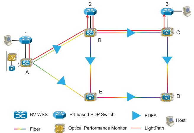
FIGURE 5. IP-over-optical network testbed used for experimental demonstrations.
