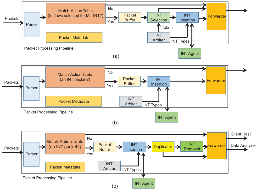
FIGURE 3. Packet processing pipelines designed for realizing flexible ML-INT in (a) the ingress switch, (b) an intermediate switch, and (c) the egress switch.
