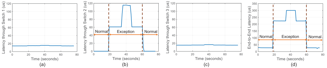
FIGURE 9. Results for the first use-case, (a) packet queuing latency at Switch 1 , (b) packet queuing latency at Switch 2 , (c) packet queuing latency at Switch 3 , and (d) end-to-end latency measured by commercial traffic analyzer.
