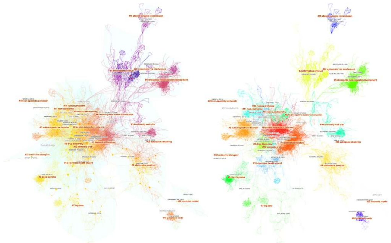
Fig 7. A network visualization based on the combined dataset, featuring 3,095 references and 16,314 co-citation links. Modularity: 0.84. Silhouette: 0.34.
