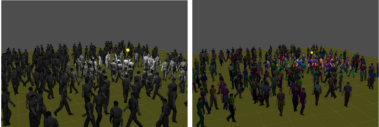
Figure 10: Adding lighting and color information to the animated impostors.
