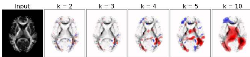
Figure 12: How the patch size influences the visualization. For the input image (HIV sample, slice 39 along the first axis) we show the visualization with different patch sizes ( k in alg. 1). Prediction differences are shown only for voxels with (absolute) relevance value above 15% of the (absolute) maximum (for k = 2 it is 10%).
