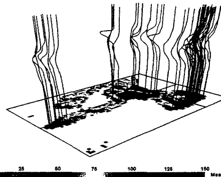
Fig. 10. Same query results as shown in Figure 9 except that the pdfs are plotted directly above the corresponding grid cells. These pdf curves provide another visual cue of the distributions found by a mode query.
