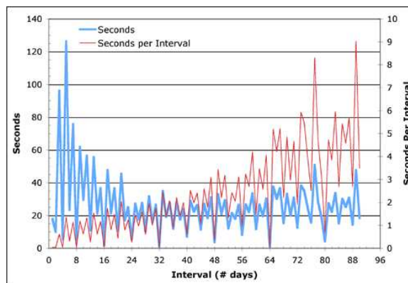
Figure 10: Average time taken as a function of window size.
