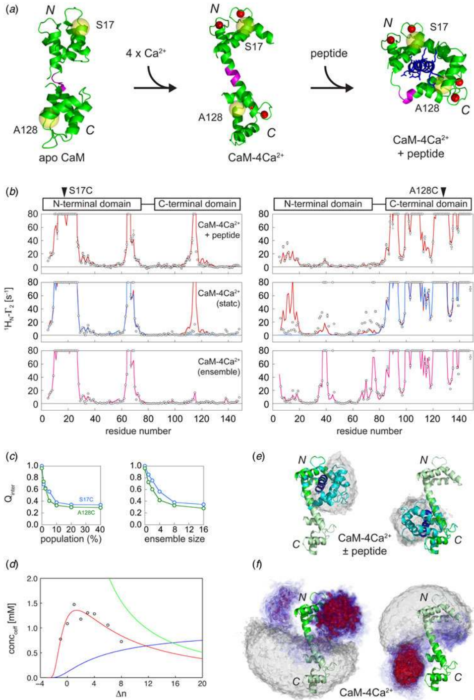
Fig. 9. Visualizing sparsely populated compact ‘dark’ states in Ca 2+ activation of CaM. (a) Structures of CaM in various physiological states. Ca 2+ ions are shown as red spheres, and spin-labeling sites S17C and A128C are indicated by yellow spheres. The flexible linker (residues 77–81) is shown in magenta. (b) Experimental PRE profiles for Ca 2+ -loaded CaM (with a spin label at S17C or A128C), in the presence or absence of peptide, are shown as circles (error bar, 1 s.d.). PREs too large (>80 s -1 ) to be accurately
