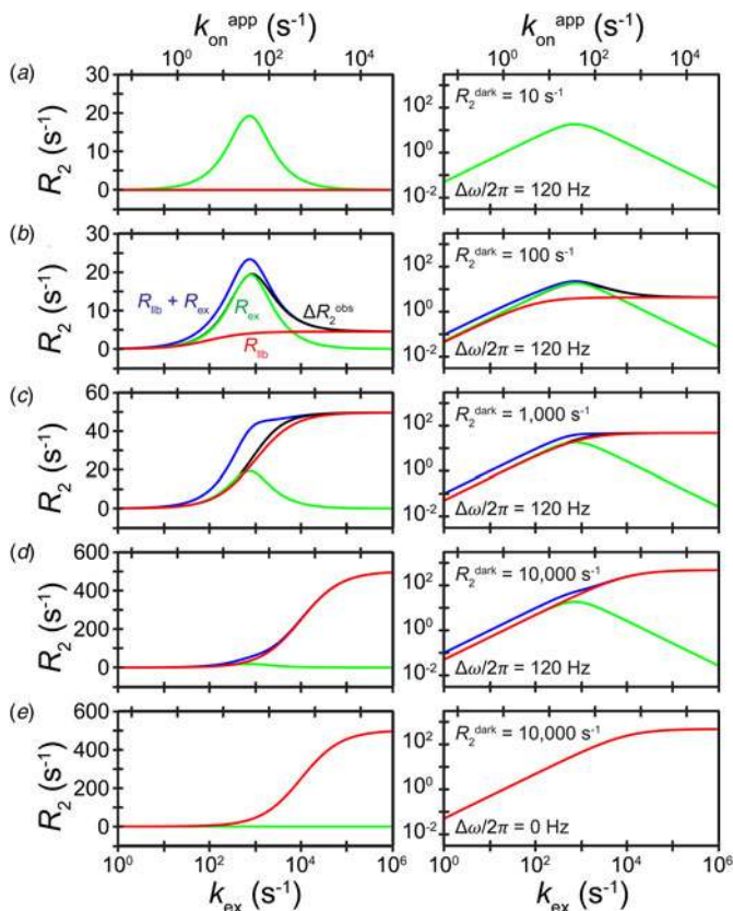
Fig. 5. Enhanced apparent observed transverse relaxation rate ( R_2^{\text{obs}} ) due to exchange with a minor species. Lifetime line broadening ( R_{\text{illb}} , red), chemical shift exchange broadening ( R_{\text{ex}} , green), their sum ( R_{\text{illb}} + R_{\text{ex}} , blue), and the observed enhancement in apparent transverse relaxation rate ( \Delta R_2^{\text{obs}} , black) compared with a system in the absence of exchange are plotted versus exchange rate. Curves are shown for a small, rapidly tumbling visible species ( p_A = 95\% , R_{2,A}^0 = 10 \text{ s}^{-1} ) in exchange with a sparsely populated ‘dark’ state ( p_B = 5\% ). On the left, simulated data are plotted using a linear scale for the y -axis (note that the scale varies between plots); on the right, a logarithmic scale is used for the y -axis (same scale in all plots); the x -axis is plotted with a logarithmic scale in all instances. The x -axis on the top of the plot shows the apparent first-order rate constant ( k_{\text{on}}^{\text{app}} or k_{\text{AB}} ) for molecules of state A going to state B. The x -axis on the bottom of the plot shows the overall exchange rate ( k_{\text{ex}} = k_{\text{on}}^{\text{app}} + k_{\text{off}} = k_{\text{AB}} + k_{\text{BA}} ). (a) In the absence of a difference in R_2^0 between the two states, only R_{\text{ex}} is observed for a system with a difference in chemical shifts between the two states, which has a maximum value when k_{\text{ex}} = \Delta\omega . Here, \Delta\omega/2\pi = 120 \text{ Hz} (e.g. 2 ppm for ^{15}\text{N} in a 600 MHz static field). (b–d) If the two states differ in chemical shift and state B exhibits a faster transverse relaxation time – i.e. for a high-molecular-weight, slowly tumbling dark state – then \Delta R_2^{\text{obs}} will have contributions from both R_{\text{ex}} and R_{\text{illb}} . In the slow exchange regime ( k_{\text{ex}} \ll R_{2,B} - R_{2,A} and k_{\text{ex}} \ll \Delta\omega ), \Delta R_2^{\text{obs}} = R_{\text{ex}} = R_{\text{illb}} = k_{\text{on}}^{\text{app}} . In the fast exchange regime ( k_{\text{ex}} \gg R_{2,B} - R_{2,A} and k_{\text{ex}} \gg \Delta\omega ), \Delta R_2^{\text{obs}} = R_{\text{ex}} + R_{\text{illb}} , and under very fast exchange, the value of R_{\text{ex}} approaches zero, and R_{\text{illb}} approaches a population-weighted maximum value (e.g. in panel (d), \Delta R_2^{\text{max}} = 500 \text{ s}^{-1} = 5\% \times 10\,000 \text{ s}^{-1} ). Note that the same curve for R_{\text{ex}} is shown in panels (a–d). (e) In the absence of a difference in chemical shift between the two states, only R_{\text{illb}} is observed for a system with a difference in R_2^0 between the two states. For all panels, R_2^{\text{obs}} was determined by first solving the McConnell equations to generate a magnetization time course, which was then fit to the free induction decay of a single resonance with R_2^{\text{obs}} . A similar procedure was carried out to determine R_2^{\text{obs}} in the absence of R_{\text{illb}} ( R_2^{\text{obs}}[R_{2,B} = R_{2,A}] ) and in the absence of R_{\text{ex}} ( R_2^{\text{obs}}[\Delta\omega = 0] ). Values were calculated as follows for each exchange rate: \Delta R_2^{\text{obs}} = R_2^{\text{obs}} - R_{2,A} , R_{\text{illb}} = R_2^{\text{obs}}[\Delta\omega = 0] - R_{2,A} , and R_{\text{ex}} = R_2^{\text{obs}}[R_{2,B} = R_{2,A}] - R_{2,A} . All calculations were performed in MATLAB.
