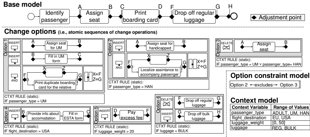
Figure 24: Provop model of the check-in process
