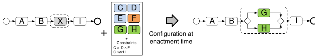
Figure 16: Configuring a specific region of a process variant at enactment time
