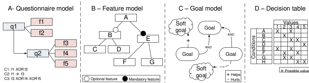
Figure 15: Example of configuration techniques
