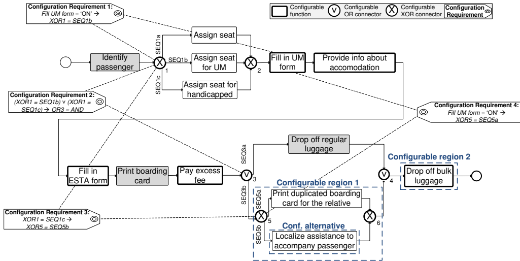
Figure 23: Configurable process model of the check-in process (in C-EPC notation)
