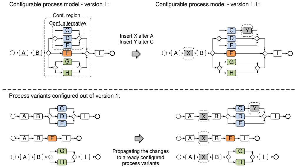
Figure 19: Propagating changes between configured process variants
