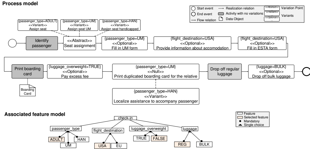
Figure 25: PESOA model of the check-in process
