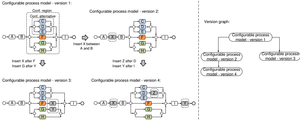
Figure 18: Versioning of a configurable process model
