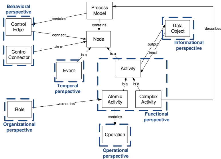
Figure 3: Process meta-model adopted from [22]
