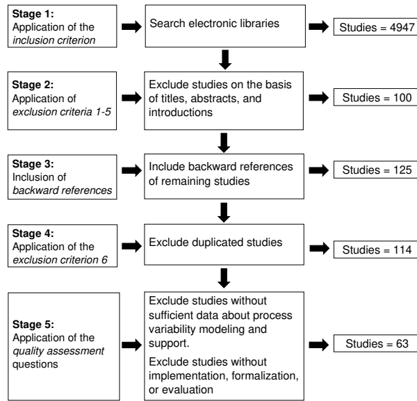
Figure 5: Stages of the study selection process
