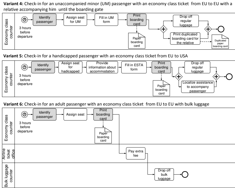
Figure 2: Variants of the check-in process (2)
