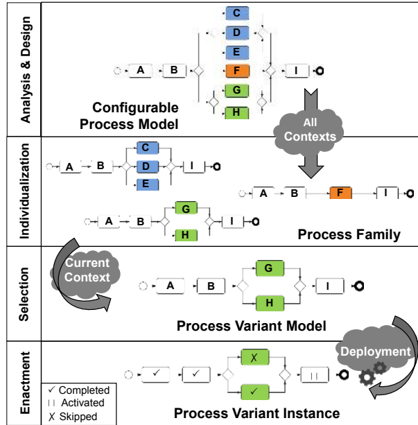
Figure 4: From process family definition to process variant enactment
