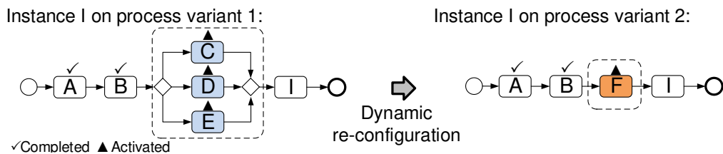
Figure 17: Dynamically re-configuring an instance of a process variant
