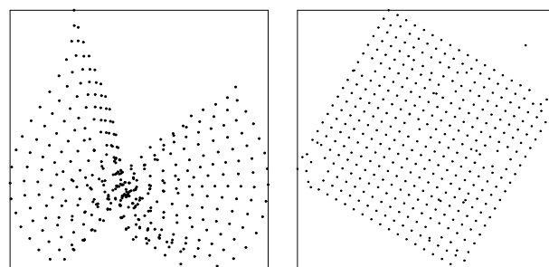
Figure 7: A pathological case showing the possible effect of communication patterns on the chosen coordinates. In the first case, nodes only contact their four nearest neighbors, allowing the resulting coordinates to twist over long distances. In the second case, nodes contact distant nodes as well, improving the accuracy of the coordinates at the larger scale.
