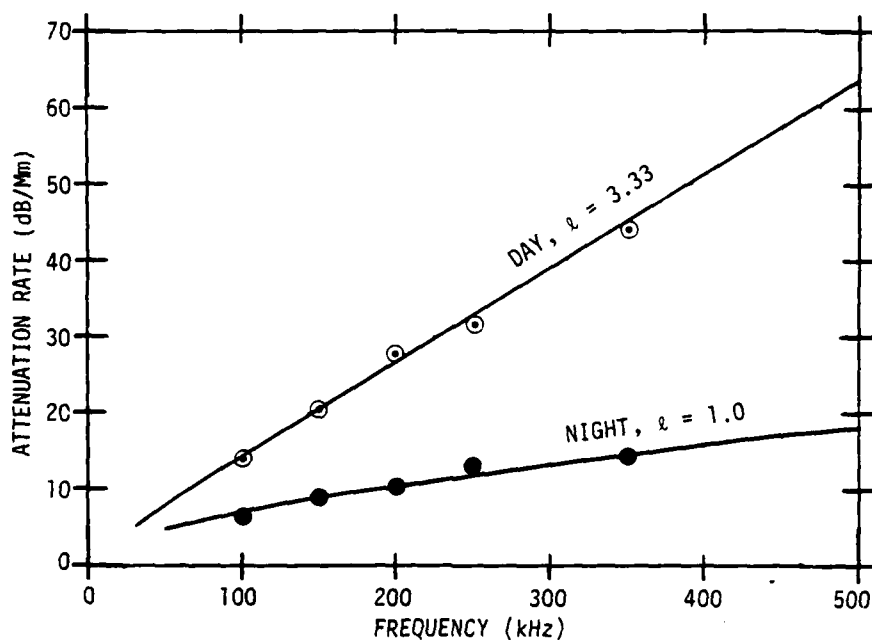
Figure 8. Comparison of Attenuation Rate Versus Frequency (Daytime l = 3.33 km and Nighttime l = 1.0 km)
