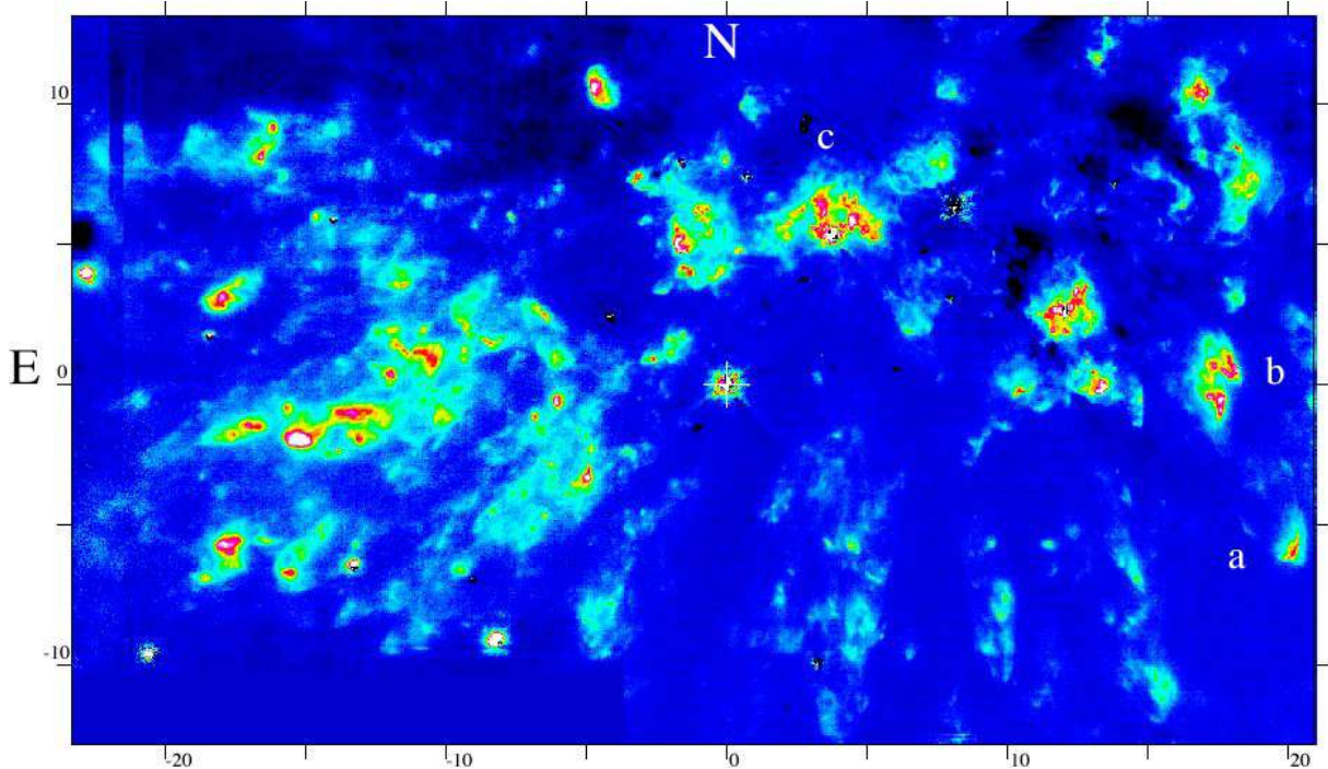
Fig. 1. H 2 emission in the 1–0 S(1) line at 2.121 \mu\text{m} , with continuum emission subtracted. Image size: 44.5'' \times 26''. The cross indicates the position of the star TCC016 (05 h 35 m 14 s .91, –05°22'39".31 (J2000)) and a,b,c identify objects shown in more detail in subsequents. The SE and ESE frames, referred to in the text, are respectively the regions to the west and to the east of TCC0016.
