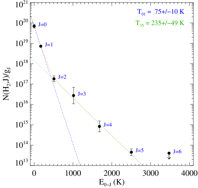
Fig. 13. Excitation diagram of H_2 towards J2140–0321. The straight blue (resp. green) dotted line corresponds to the excitation of the low (resp. high) rotational levels. The orange curve correspond to the sum of the two populations in Boltzmann equilibrium at the two different temperatures.
