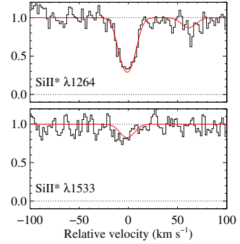
Fig. 16. Si II* at z_{\text{abs}} = 2.34 towards J2140–0321. The absorption at +50 \text{ km s}^{-1} in the Si II* \lambda 1264 panel is due to Si II* \lambda 1265 .
