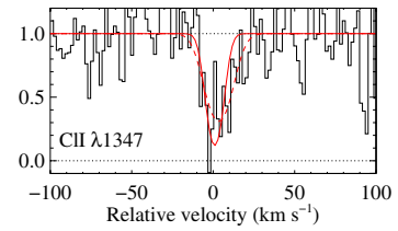
Fig. 11. Neutral chlorine in the DLA at z_{\text{abs}} = 2.34 towards J2140–0321. The dashed profile corresponds to a fit with all parameters free, while b is fixed to that of ClI for the solid profile.
