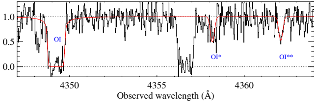
Fig. 15. Neutral oxygen fine-structure lines in the DLA at z_{\text{abs}} = 2.34 towards J2140–0321. The absorption lines seen at \lambda \approx 4348 and 4356.5 \text{ \AA} correspond to \text{OI}\lambda 1301 and \text{Si II}\lambda 1304 , respectively.
