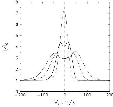
Fig. 6. Normalized Bry line profiles of the disk-wind model 5 from Table A.1 at the inclination angles i = 10^\circ (dotted line), 20^\circ (solid), 40^\circ (dashed), and 60^\circ (dashed-dotted; high spectral resolution, not degraded to the spectral resolution of AMBER).
