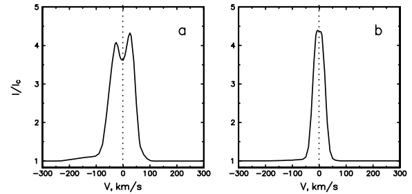
Fig. A.7. Bry line profile of model 4 with constant a) and outward decreasing b) parameter f ( i = 20^\circ ; see Sect. A.4.1 for details).
