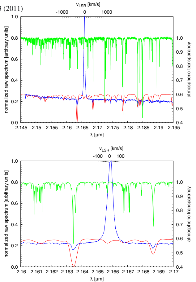
Fig. B.1. Wavelength calibration of the AMBER data. Top : raw AMBER spectrum of MWC 297 (solid blue line) compared to a telluric spectrum from the Kitt Peak Observatory. The green line shows the original Kitt Peak spectrum with a spectral resolution of 60 000, while the red line displays the telluric spectrum that has been convolved to the same spectral resolution as the AMBER data ( R = 12\,000 ). For clarity, the red curve has been shifted down by 0.4. As the figure reveals, after the wavelength calibration, the AMBER raw spectrum of MWC 297 matches several telluric features. Bottom : same as top panel, but just for the wavelength region around the Bry line.
