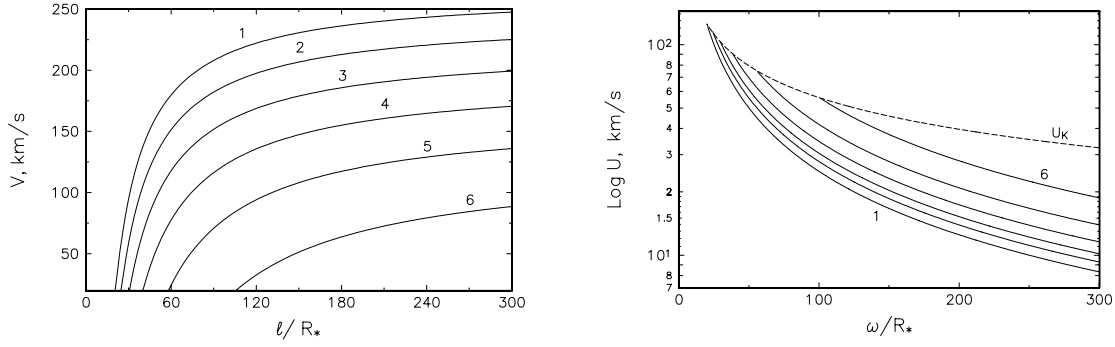
Fig. A.2. Left: radial velocity of the outflow along the different streamlines as a function of l ; numbers 1–6 denote the number of the streamline. Right: the same for the rotational velocity; the dashed line shows the Keplerian velocity in the disk.
