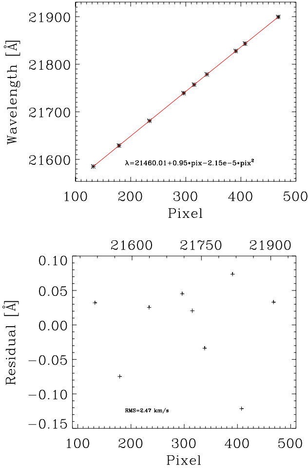
Fig. B.2. Top : calibration between the pixel and wavelength values of the VLTI/AMBER observations of MWC 297. A least-square polynomial fit of the data is also shown (red line). Bottom : residuals between the measured position of the telluric line spectrum obtained from the wavelength calibration of the AMBER data and the expected position from the reference telluric spectrum provided by NOAO. The root-mean square value is of the order of 2.5 \text{ km s}^{-1} .
