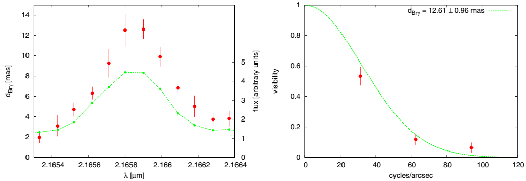
Fig. 3. Left: Gaussian FWHM fit diameters of the Bry line-emitting region for several individual spectral channels (in the center and the line wings) across the Bry emission line (red bullets). The diameters are derived from continuum-compensated visibilities. Therefore, they are the diameters of the Bry line-emitting region and not of the emission region of both line plus continuum. The AMBER spectrum of MWC 297 is shown for comparison (green curve). Right: Gaussian fit to the continuum-compensated AMBER visibilities at the peak intensity of the Bry emission line.
