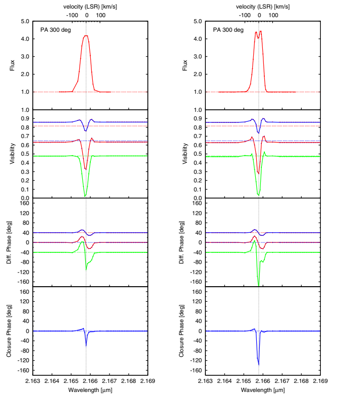
Fig. A.3. Comparison of the theoretical interferometric quantities of model 5 obtained with ( left ) and without ( right ) modeling of AMBER's spectral resolution of 12 000. In both cases, position and inclination angles are identical (PA = 300°, i = 20^\circ ).
