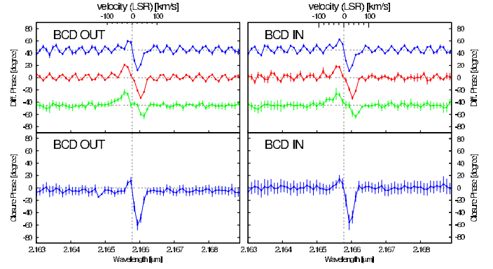
Fig. C.1. Differential phases and closure phases derived from the data obtained without ( left , BCD OUT) and with ( right , BCD IN) the beam commutation device. The shown signals are not yet corrected using the calibrator data. After we corrected the sign changes introduced by the BCD device, the two data sets yield the shown signals, which are nearly identical and demonstrate the high accuracy of the measured phase signals.
