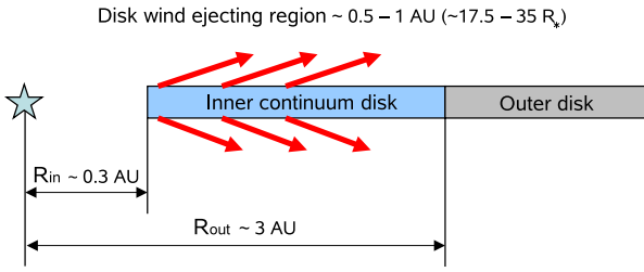
Fig. 4. Sketch of the MWC 297 disk-wind model adopted in this paper.
