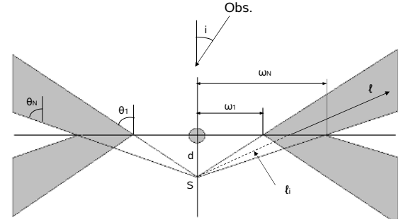
Fig. A.1. Sketch of the geometry of the disk-wind model adopted.
