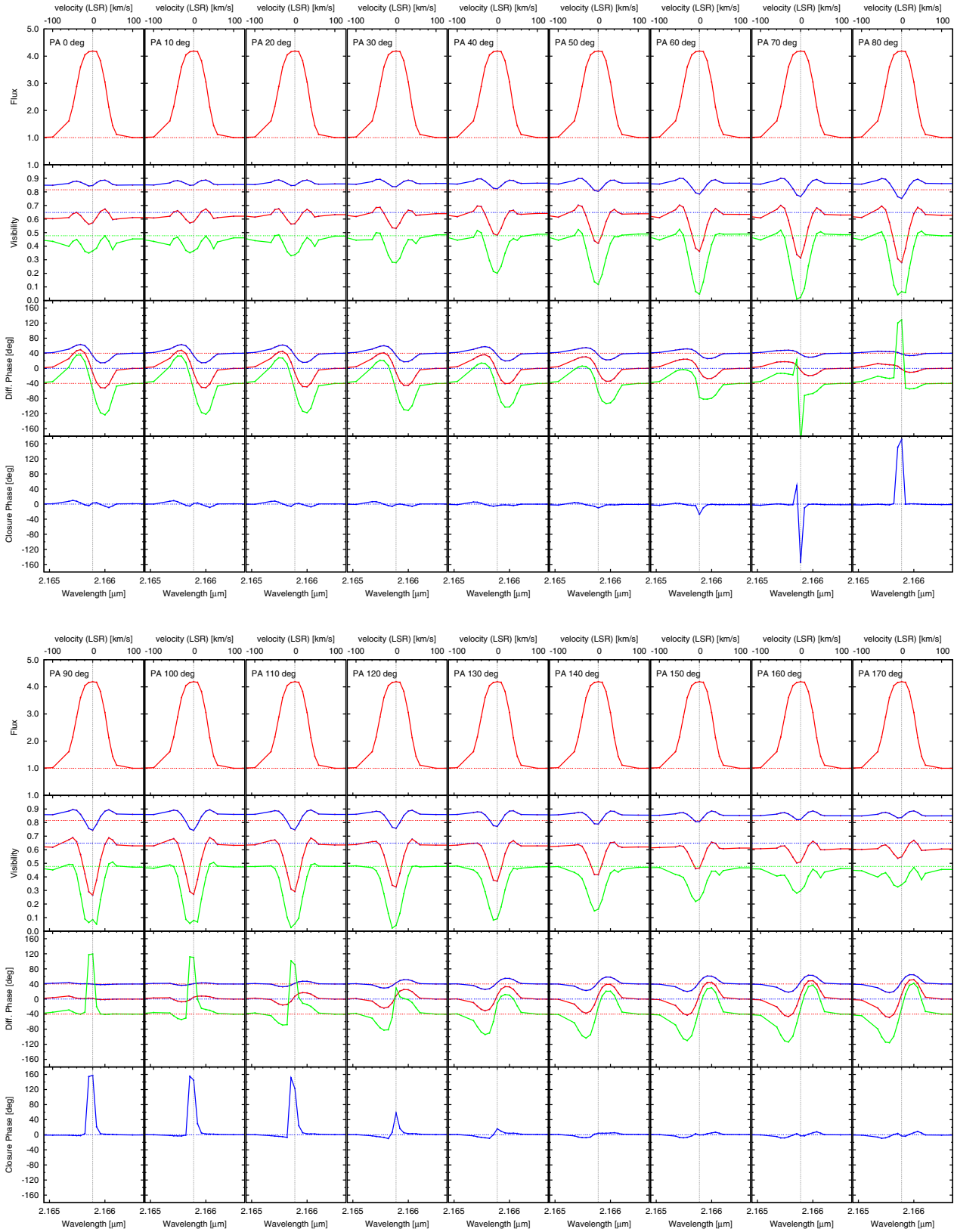
Fig. A.4. Dependence of the visibilities and phases of model 5 (see Tables 3 and A.1) on both the wavelength across the Bry line and the PA of the model on the sky for an inclination angle of i = 20^\circ and clockwise motion of the disk wind (the corresponding anti-clockwise plots are shown in Fig. A.5). Top: PAs from 0 to 80^\circ in steps of 10^\circ from left to right; bottom: PAs = 90 to 170^\circ . Closest agreement between observation and model is obtained for PAs of 65, 120, 245, and 300^\circ , as discussed in Sect. A.3.
