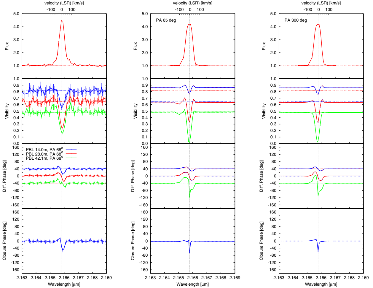
Fig. 7. Comparison of the observations ( left panel ; see Fig. 1) with the corresponding model quantities of model 5 for two different PAs of the model image ( middle and right panel ; the model quantities are calculated for AMBER’s spectral resolution of 12 000, as discussed in Sect. A.3 and Fig. A.3). The middle and right panels show the dependence of the interferometric observables (spectrum, visibilities, wavelength-differential phases, and closure phases) of our best-fit disk-wind model 5 (disk-wind emitting region, continuum accretion disk, plus central star; Tables 3 and A.1) on the wavelength across the Bry line for an inclination angle of i = 20^\circ , clock-wise motion of the disk wind, and for two different PAs of the projected disk polar axis on the sky: 65^\circ ( middle ) and 300^\circ ( right ). Several other PAs that are also approximately in agreement with the observations are discussed in the text and Figs. A.4 and A.5. The detailed dependence of the interferometric observables on the PA is presented in Figs. A.4 and A.5.
