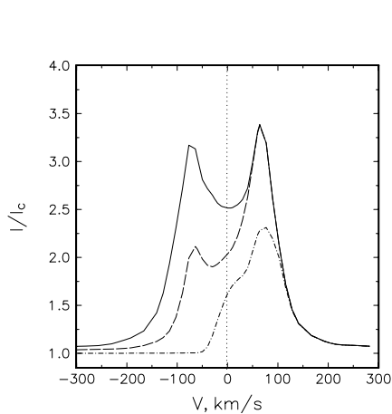
Fig. A.8. Dependence of the Bry line profile on screening caused by an optically thick, dusty disk wind. The solid line represents the unscreened line profile of model 2 (see Table A.1) with f = 5 , while the long-dashed ( H_d = 100 R_* ; \theta = 20^\circ ) and dot-dashed ( H_d = 130 R_* , \theta = 25^\circ ) lines show models with screening. For all models shown, the inclination angle is i = 70^\circ . See text for further details.
