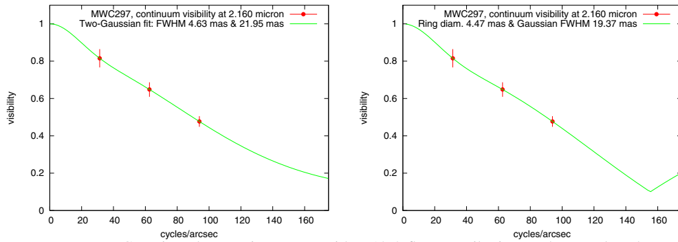
Fig. 2. Left: fit of a two-component Gaussian plus a point source with a 10% flux contribution to the wavelength-averaged (2.147–2.194 \mu\text{m} ) K -band continuum visibilities near Bry. Right: fit of a compact ring plus Gaussian halo plus a point source with a 10% flux contribution to the K -band continuum visibilities.
