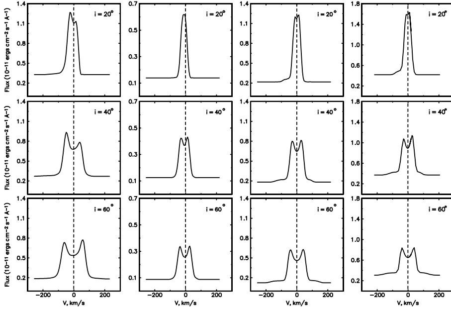
Fig. A.6. Disk-wind model profiles of the Bry line for different inclination angles (from top to bottom: 20, 40, and 60°). From left to right, the profiles correspond to models 1, 2, 3, and 4 in Table A.1 (model 5 is discussed in Fig. 6).
