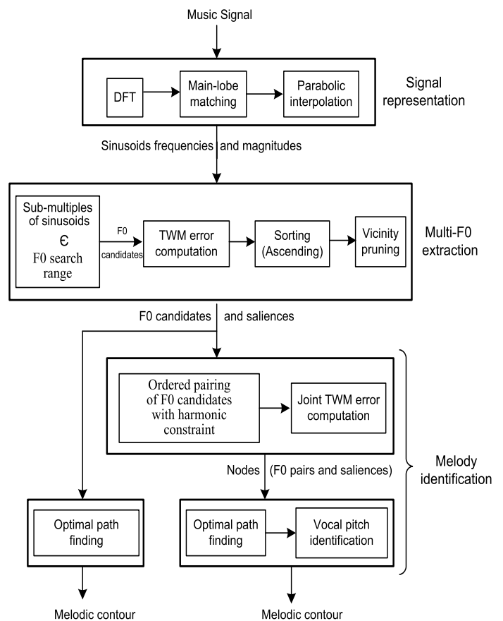
Fig. 2. Block diagram of proposed system
