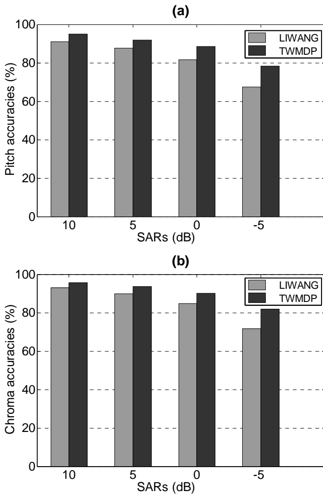
Fig. 3. (a) Pitch and (b) Chroma accuracies for LIWANG and TWMDP Single-F0 tracking systems for Dataset 1 at SARs of 10, 5, 0 & -5 dB.
