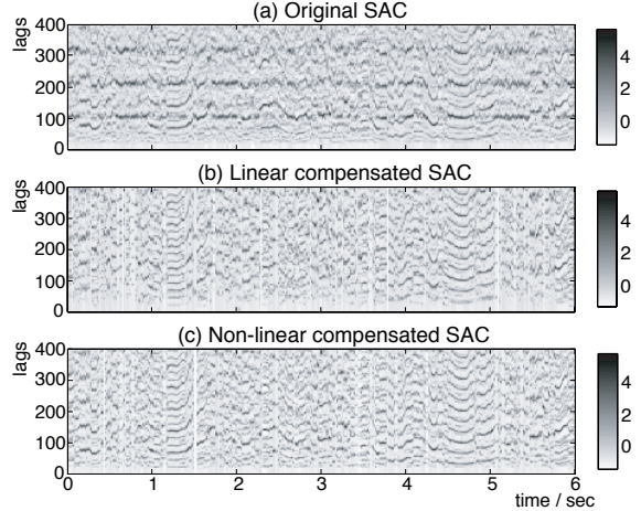
Figure 3: SACs for the input signal from figure 1 with and without compensation using the local-average ACF over a 1 s window. Stationary harmonic air-conditioning noise appears as a sequence of strong peaks at lags of 105, 210 and 315 samples in the original SAC, but is clearly deleted in the non-linear compensated SAC (panel (c)), which also preserves speech information lost in the linear compensated SAC of panel (b). The non-linear compensated SAC is the basis of the enhanced pitch tracks shown in figure 1 (d).
