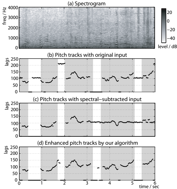
Figure 1: Example of noisy speech from a personal audio recording. The pitch tracks in (b) and (c) are extracted by a noise-robust PDA as described in the text; pane (d) shows the result of our algorithm with the same input signal. The pitch of a stationary periodic air-conditioning noise appears as flat contours around lags 105 and 210 in (b), and tends to be more dominant around 4-6 s in (c) due to the failure of a noise estimation of the spectral subtraction, but is clearly deleted by our method in (d). Shadowed regions indicate manually-labeled voiced segments.
