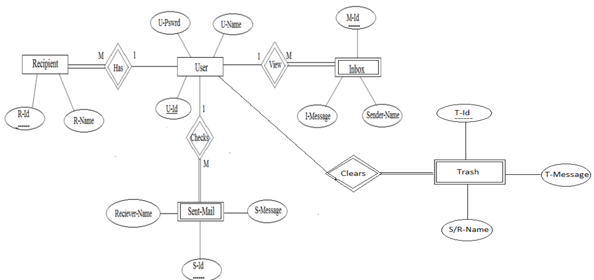
Fig. 1. E-R Diagram of our system
