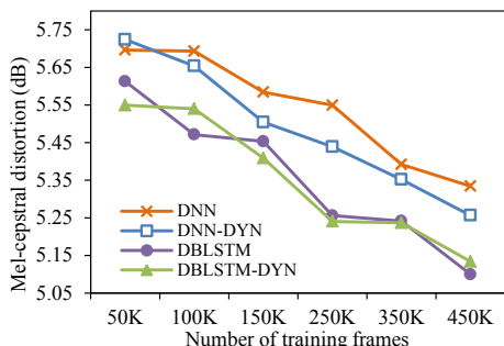
Fig. 6. Mel-cepstral distortion for each method. The smaller MCD value is, the closer the converted spectra is to the target spectra.
