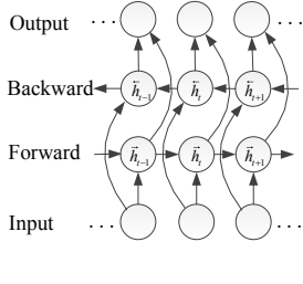
Fig. 1. Bidirectional RNNs
