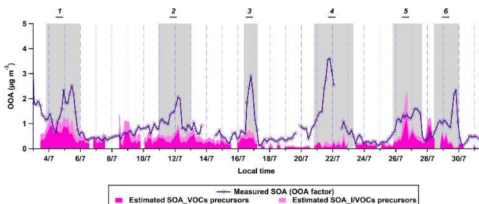
Figure 8. Temporal evolution of the OOA, or SOA, concentrations ( \mu\text{g m}^{-3} ) (1) observed at SIRTa, (2) estimated from the VOCs and (3) from the I/VOCs (i.e., VOCs+C 12 –C 16 IVOCs) measured at SIRTa using atmospheric-relevant SOA yields. The grey-shaded areas highlight the “Atlantic Polluted” wind regimes associated with stagnant conditions and increased OOA.
