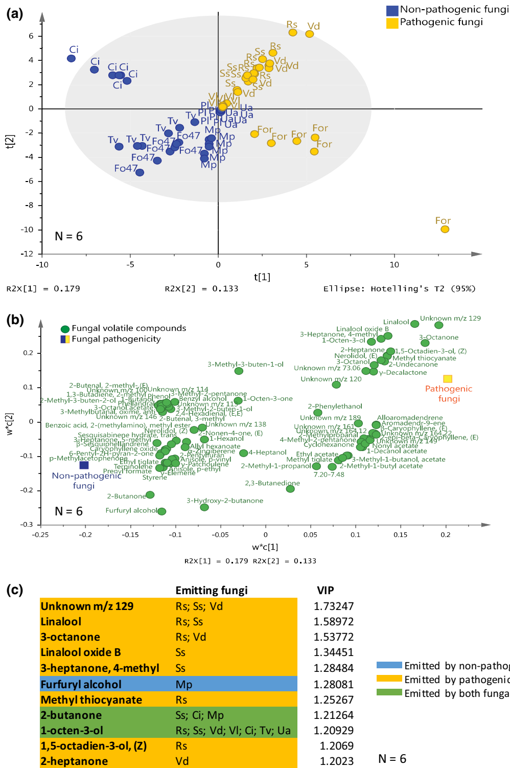
Fig. 1 Projection to Latent Structures Discriminant Analysis (PLS-DA) of volatile organic compounds (VOCs) collected from the headspace of pathogenic and non-pathogenic fungi of Arabidopsis thaliana . a Grouping pattern of samples according to the first two principal components and the Hotelling's T2 ellipse confining the confidence region (95%) of the score plot. b Contribution of individual VOCs to the first two principal components is shown in the loading plot of the PLS-DA. c List of VOCs with values of variable
