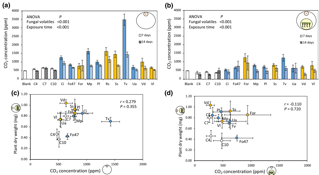
Fig. 6 CO 2 concentration (mean ± SE) measured for the 11 fungi and their respective controls when a enclosed alone, and b co-cultivated with Arabidopsis thaliana seedlings for 7 and 14 days. Pearson correlation between the average plant dry weight (mean ± SE) upon co-cultivation for 14 days and c the average CO 2 concentration (mean ± SE) measured after 14 days when the fungi were enclosed alone, and d the average CO 2 concentration (mean ± SE) measured after 14 days when the fungi were co-cultivated with plants. Blank, empty Petri dish; C4, C7 and C10, medium alone pre-incubated for 4, 7, and 10 days; Ci, Chaetomium indicum ; Fo47, Fusarium oxysporum 47; For, F. oxysporum f.sp. raphani ; Mp, Mucor plumbeus ; Pl, Phoma
