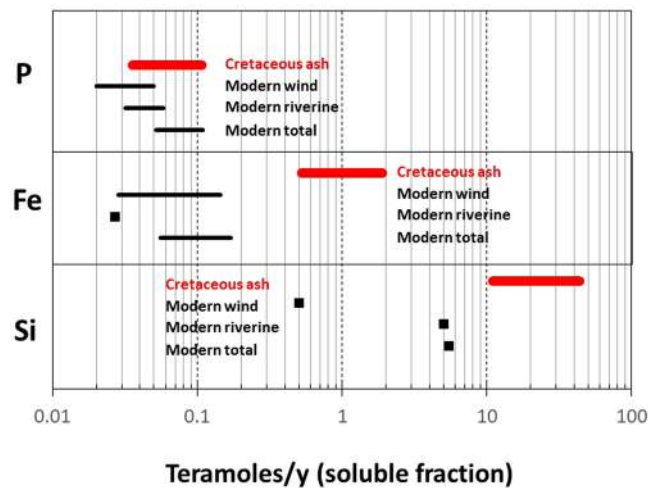
Figure 4. Estimated inputs of soluble Si, Fe and P in Teramoles/y. Red bars represent soluble flux from Cretaceous windblown ash only (this study). Black lines or squares represent soluble inputs into ocean for wind, riverine and combined riverine + wind in the present day (P from Table 3 in Ruttenberg 77 ; Fe from Jickells et al. 76 and Meybeck 73 ; Si from Treguer et al. 72 and Meybeck 73 ). Details of calculations are discussed in the text.
