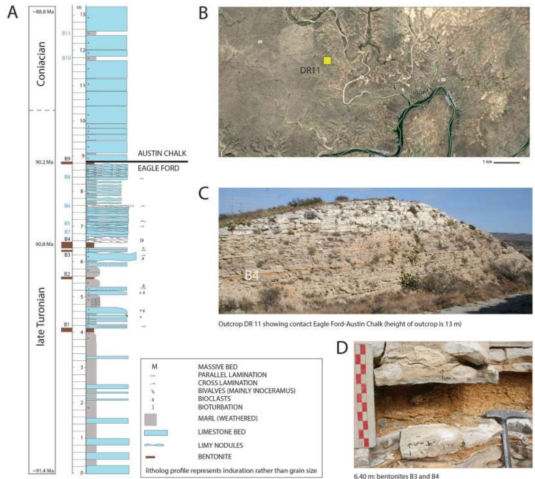
Figure 2. Field site in west Texas. (A) Stratigraphic section of outcrop DR11 modified from Minisini et al. 56 . Discrete ash layers noted as brown and denoted with black font in the stratigraphic column, while marls with disseminated ash are noted in blue font. (B) Exact location of outcrop DR11. Image is from Google Earth (© Google, DigitalGlobe, CNES/Airbus, Map data © Google, INEGI). (C) Outcrop photo with ash horizons appearing as orangish recessed layers. (D) Discrete ash layer B4 (thick) is shown for reference and refers to the thickest layer seen in the outcrop in C.
