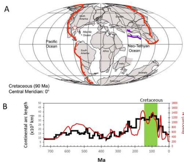
Figure 1. (A) Extent of continental magmatic arcs (red lines) above ocean-continent subduction zones in the Cretaceous map taken from Cao et al. 23 . Location of field site DR11 shown by star. (B) Length of continental arcs (black line, left vertical axis) and detrital U/Pb zircon ages (red line, right vertical axis) through time compiled from the literature 23,94 . Continental arc length is based on compilation of granitoid plutonic belts through time 23 and does not necessarily correspond with total subduction length.
