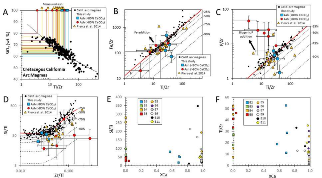
Figure 3. (A) Plutonic rock data (black circles) from the Cretaceous Peninsular Ranges Batholith in California 65 plotted as \text{SiO}_2 (wt. %) versus \text{Ti}/\text{Zr} (by weight). Red circles (thin, carbonate-rich layers) and blue squares (thick, carbonate-poor layers) represent measured \text{Ti}/\text{Zr} of ash layers. Horizontal red, orange and blue lines with arrows represent approximate \text{SiO}_2 content of protolith based on empirical correlation (curved black line) of \text{SiO}_2 versus \text{Ti}/\text{Zr} from the batholith data. (B–D) Average \text{Fe}/\text{Zr} and \text{P}/\text{Zr} versus \text{Ti}/\text{Zr} and \text{Si}/\text{Ti} versus \text{Ti}/\text{Zr} (all ratios by weight). Altered ash is given by red circles and blue squares and unaltered batholith rocks by gray open circles from this study. Curved lines represent regressions with details given in the text. Error bars represent one standard deviation. (E and F) \text{Si}/\text{Ti} and \text{Ti}/\text{Zr} (by weight) versus \text{XCa} , which is the mass fraction of Ca relative to the total mass of cations (i.e., cation mass fraction), a measure of carbonate fraction. Samples represent individual measurements, in contrast to (B–D), where only the average for each sample is shown. Blue squares in (E and F) represent thick, carbonate-poor ash horizons and red circles represent thin, carbonate-rich ash layers. Orange triangles in (A–D) represent bulk rock samples of ash horizons from 58,59 ; standard deviations are not provided for these samples because analyses represent only one bulk rock measurement.
