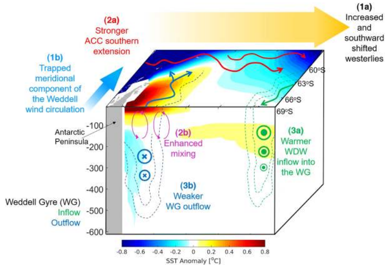
Figure 6. Schematics from the suggested mechanism in the Weddell Sea near the Antarctic Peninsula after a large eruption. The surface and vertical section in the location of SR4/WOCE stations represent the temperature anomaly for the year after the eruption (Yr + 1). The wind circulation is represented in yellow and blue thick arrows. The red arrows represent the ACC southern extension. The inflow and outflow of the WG are in green and blue, respectively. In the surface the WG is represented by the thin arrows and along the depth as dotted contours with notations for vectors coming in and out of the vertical plane.
