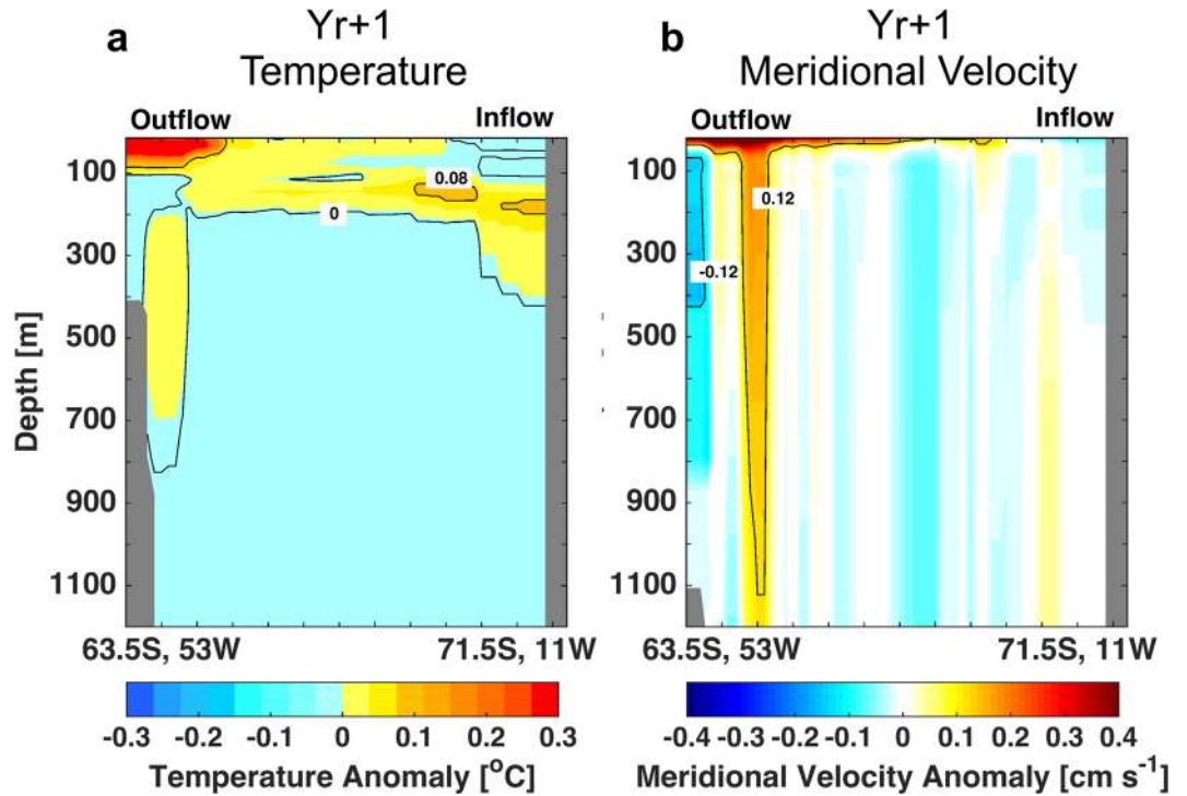
Figure 5. Depth profile composite anomalies in the year after LM eruptions (Yr + 1). (a) Potential temperature anomaly [°C]. (b) Meridional velocity anomaly [ \text{cm s}^{-1} ]. Both only shown for DJF anomalies. The transect is at the same location of SR4/WOCE stations. The inflow and outflow regions are marked, respectively 71.5°S,11°W and 63.5°S,53°W.
