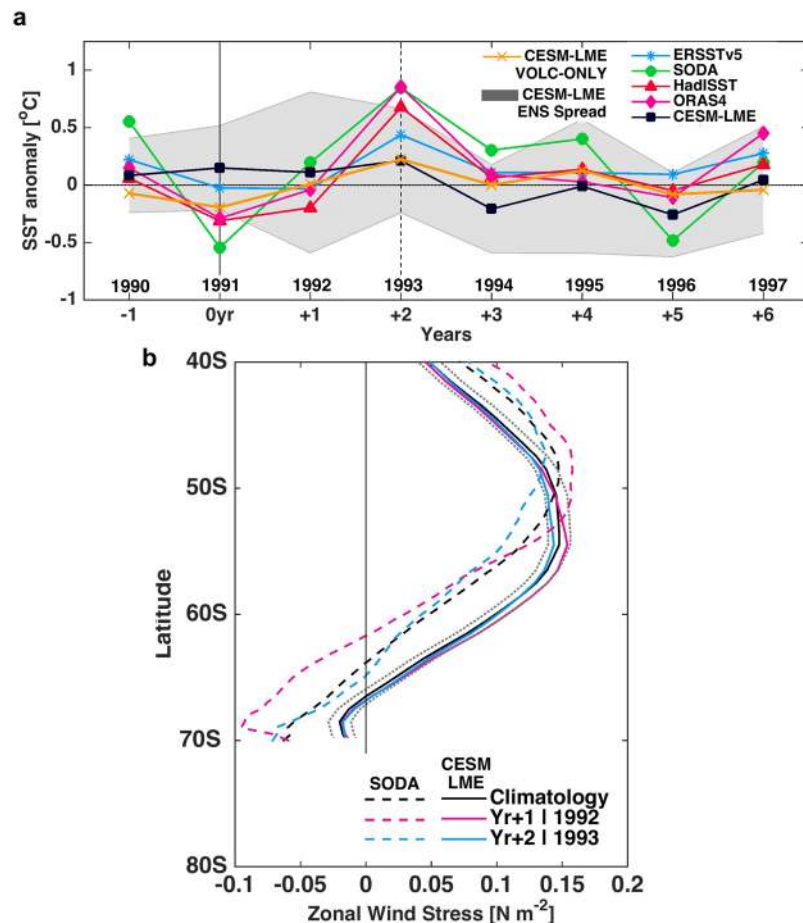
Figure 2. DJF SST anomaly time series and zonal averaged wind stress changes after Mt. Pinatubo eruption. (a) SST anomaly [ ^{\circ}\text{C} ] time series for the Antarctic Peninsula region ( 60^{\circ}\text{-}48^{\circ}\text{W} , 61^{\circ}\text{-}67^{\circ}\text{S} ). (b) Zonal averaged wind stress [ \text{N m}^{-2} ] for the South Atlantic Ocean ( 70^{\circ}\text{W} - 30^{\circ}\text{E} , 40^{\circ}\text{-}70^{\circ}\text{S} ). The dashed line represents SODA reanalysis and the continuous line CESH-LME. The grey dotted lines represent CESH-LME ensemble spread. Black lines are the climatology mean for 1980–2005.
