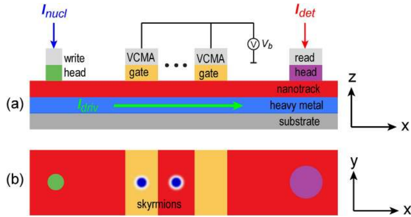
Figure 1. Schematic of the skyrmion-based racetrack memory (Sky-RM). (a) Front-view; (b) Top-view. It consists of five parts: spin-valve write head, nanotracks, magnetic tunnel junction (MTJ) read head, voltage-controlled magnetic anisotropy (VCMA) gate as well as peripheral complementary metal-oxide semiconductor (CMOS) circuits (which are not shown in the figure). The skyrmion is initially nucleated by injecting a local spin-polarized current ( I_{nucl} ) through the spin-valve write head (diameter d = 20 nm) depending on the input data, and then moves along the nanotracks (with size 1000\text{ nm} \times 80\text{ nm} \times 0.4\text{ nm} ) by the vertical spin current ( I_{driv} ). During the motion, the skyrmion can be pinned/depinned at the VCMA gate (with width of 60\text{ nm} ) by modulating the magnetic anisotropy. Finally the skyrmion can be detected by applying a detection current ( I_{det} ) across the MTJ read head due to the TMR change.
